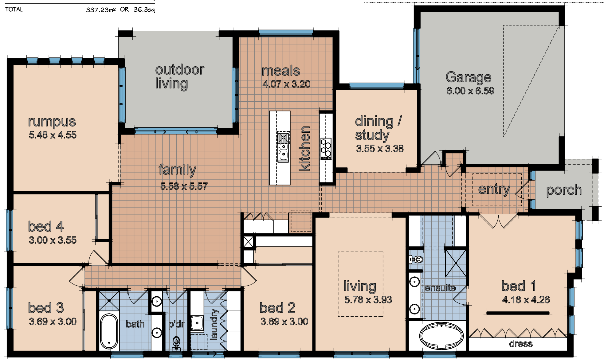
CAMBRIDGE PRESTIGE FLOOR PLAN
